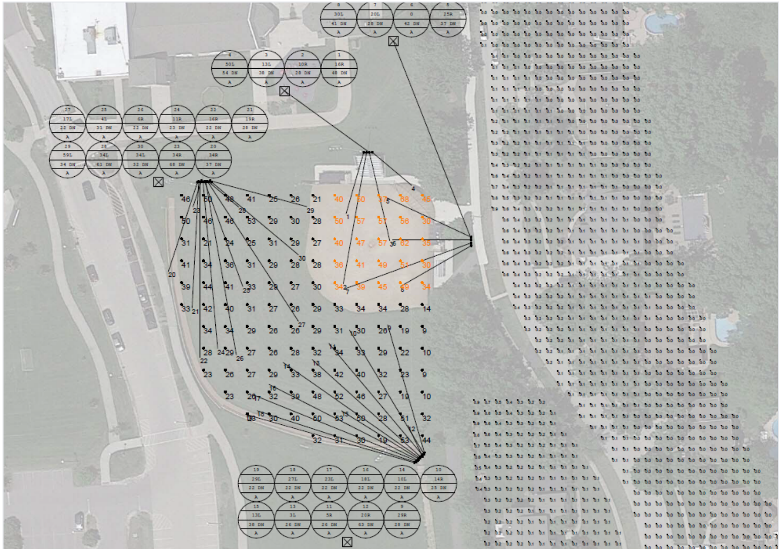
Sample photometric calculation — Baseball, 240ft, 4(65ft), Class III
